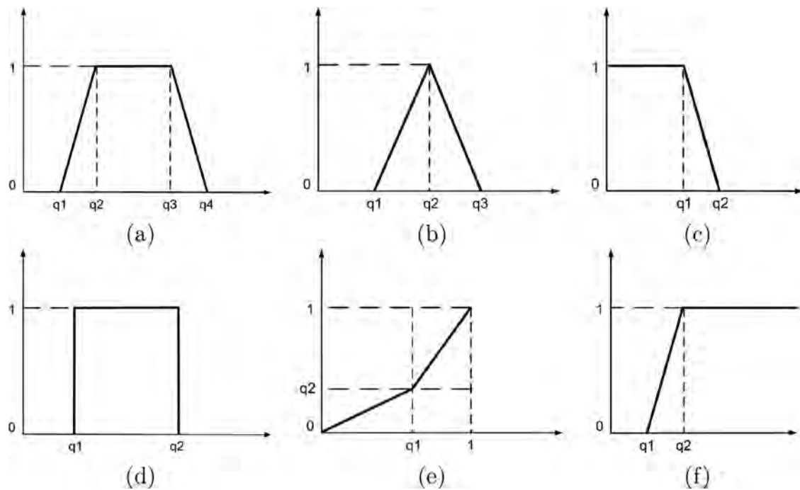
Fig. 5. (a) Trapezoidal function; (b) Triangular function; (c) Left-shoulder function; (d) Crisp interval; (e) Linear function; (f) Right-shoulder function.
