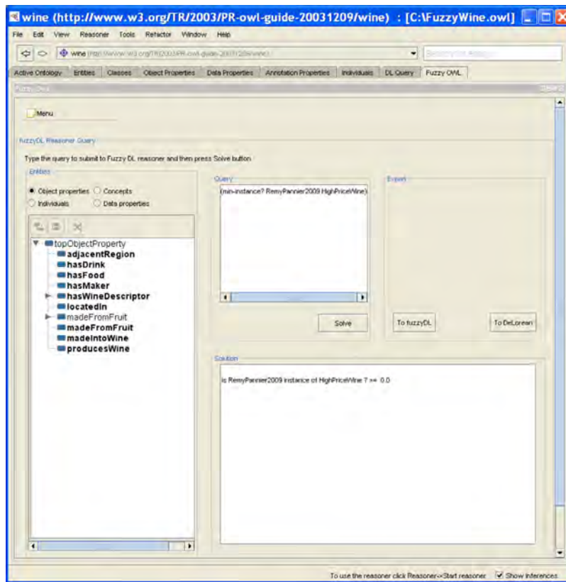
Fig. 4. Using fuzzyDL reasoner from the Fuzzy OWL 2 plug-in.
