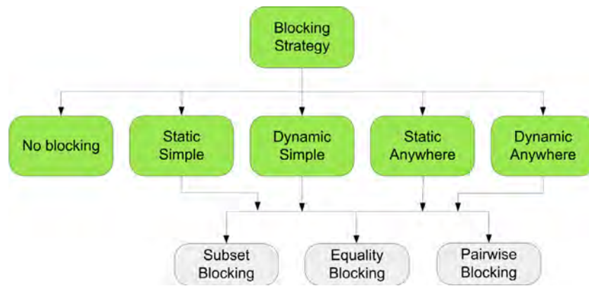
Fig. 7. Different blocking strategies implemented in fuzzyDL .
